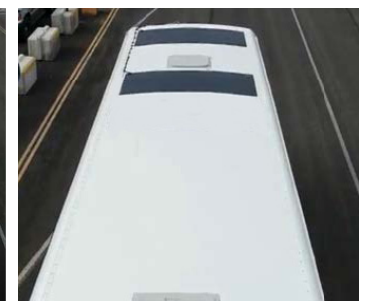
2 panel - 720W system shown
